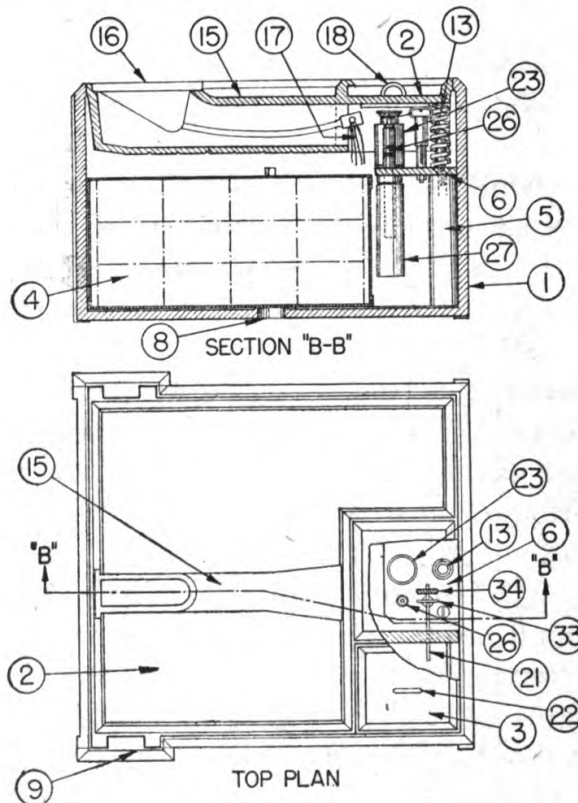
FIGURE 29.—Heavy antitank mine—plan and section.
